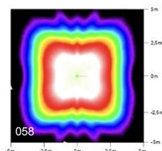
symmetrical height: 0.90m, area: 10m x 10m
