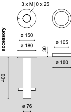
bolt-on root G180/400
